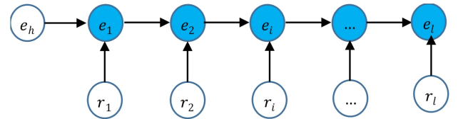
Figure 3: Recursive architecture of the Path-KCGAN generator.
