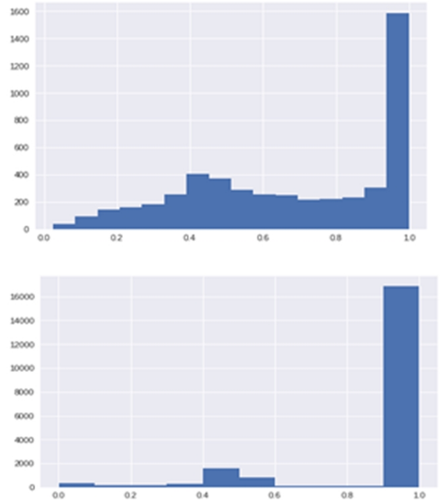
Figure 4: Distribution of predicted probabilities on WN18 and FB15k test sets.
